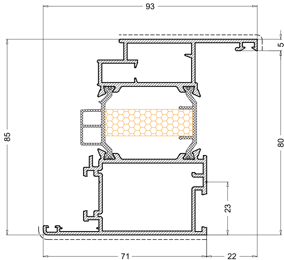
PE85214 2.046 Kg/m
