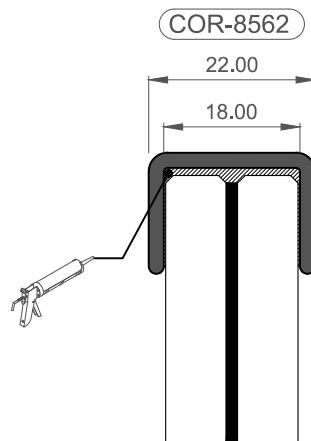
OPCIJA 1: ZATVARANJE SILIKONOM OPTION 2: SEALING WITH SILICONE
